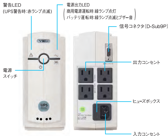
UPSmini500II
