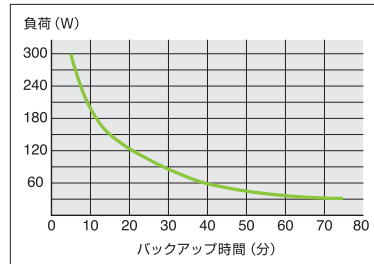
UPSmini500II
