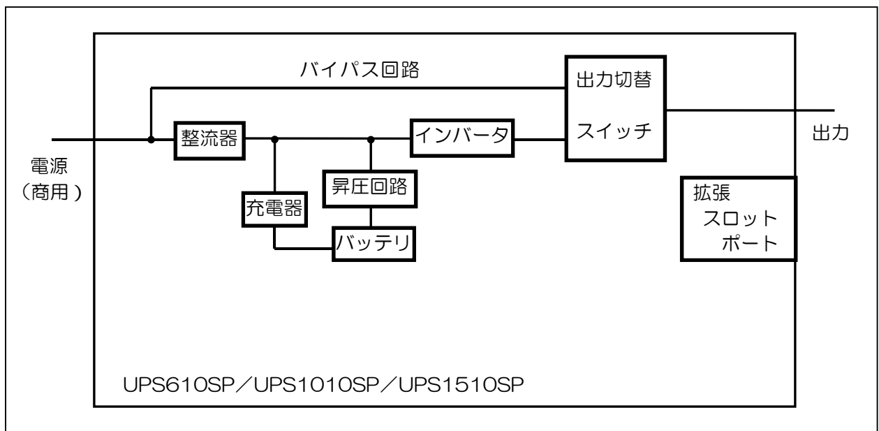
UPS610SP/UPS1010SP/UPS1510SP 概略構成図
