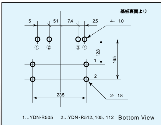
基板取付穴寸法図 PCB Installation Outlet Reference
